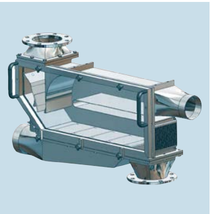
➤ HORIZONTAL FLUIDBED SEPARATOR HFS
