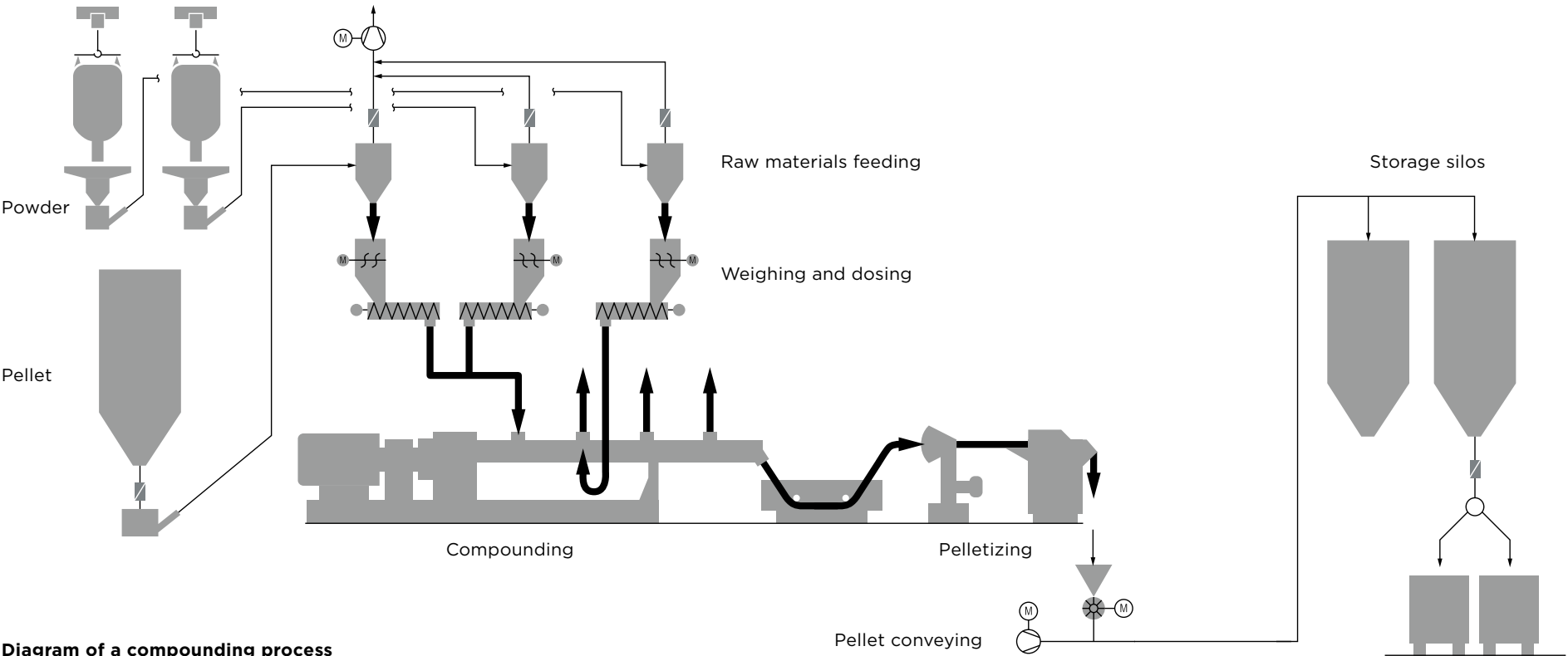
Diagram of a compounding process
