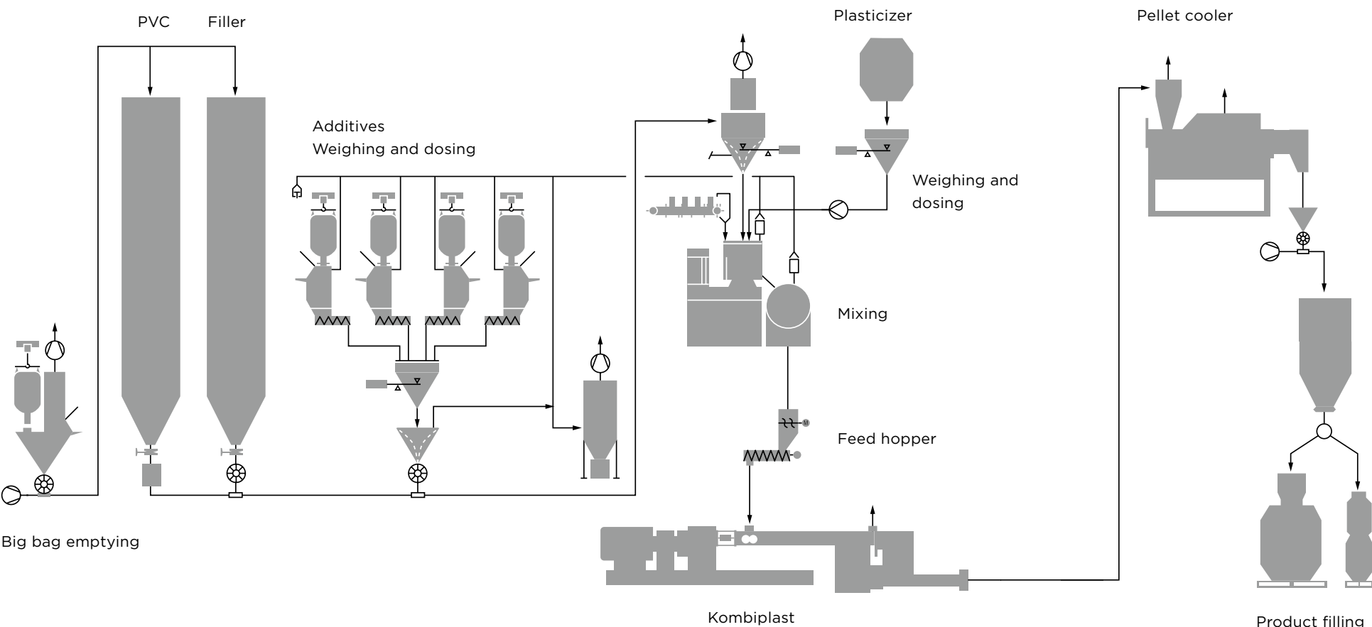
Diagram of a plastics processing process
